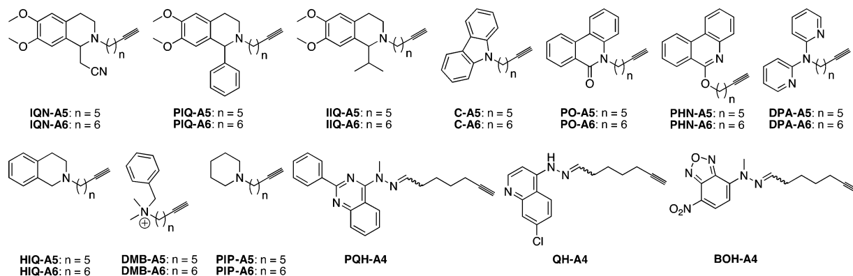
Figure 3. A library of 23 acetylene reagents in situ click chemistry screening. All chiral compounds are racemic.
