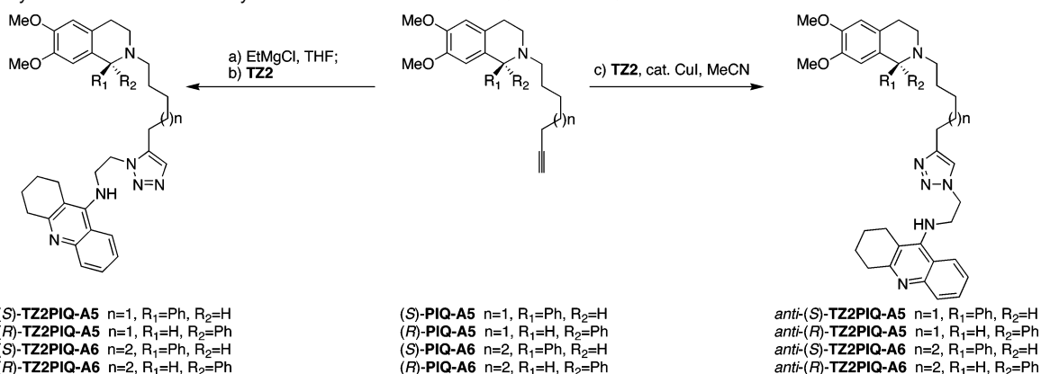
Scheme 2. Synthesis of TZ2-Derived syn - and anti -Triazoles from PIQ-A5 and PIQ-A6 a
